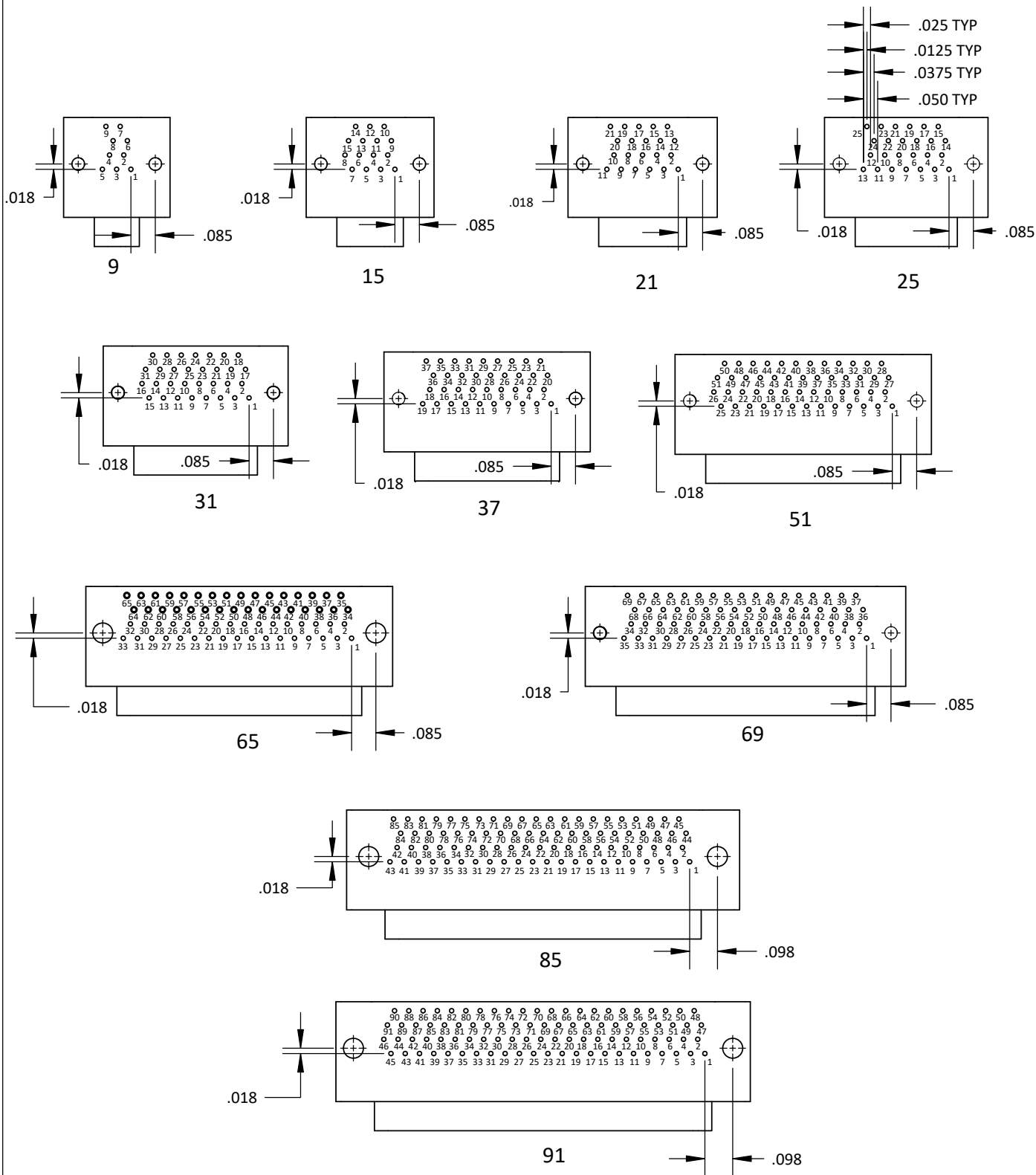
BRN2 PLUG PCB LAYOUTS .050 X .050 GRID PATTERN OFFSET .025 (EACH ROW)
