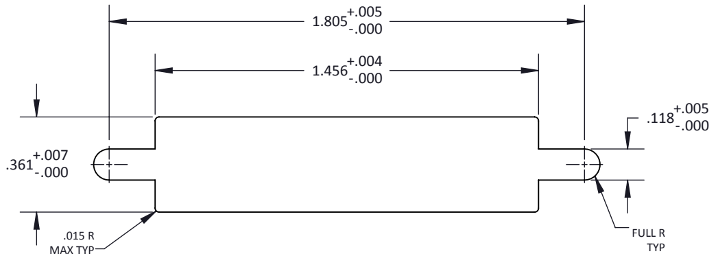
SIZES 100 FRONT PANEL CUTOUT FOR PLUG & RECEPTACLE METAL
