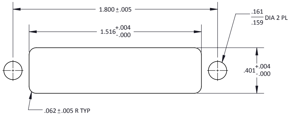
SIZES 100 REAR PANEL CUTOUT FOR PLUG & RECEPTACLE METAL
