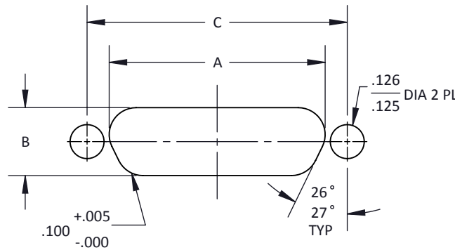
SIZES 9-69 REAR PANEL CUTOUT FOR PLUG & RECEPTACLE METAL
