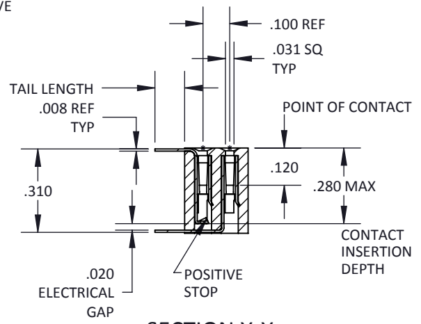
SECTION X-X
